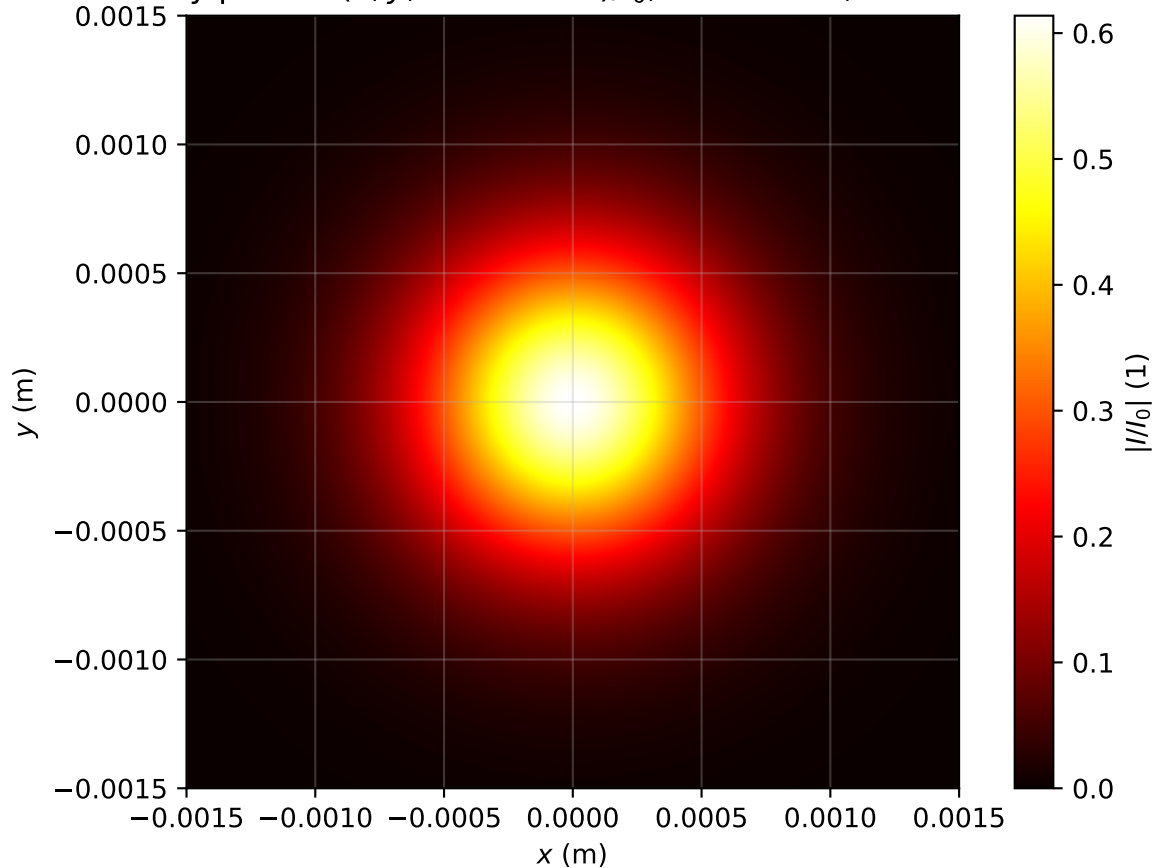
Intensity profile I(x, y, z = 2.786m)/I_0 , Pin=0.5Pcr, artificial time
